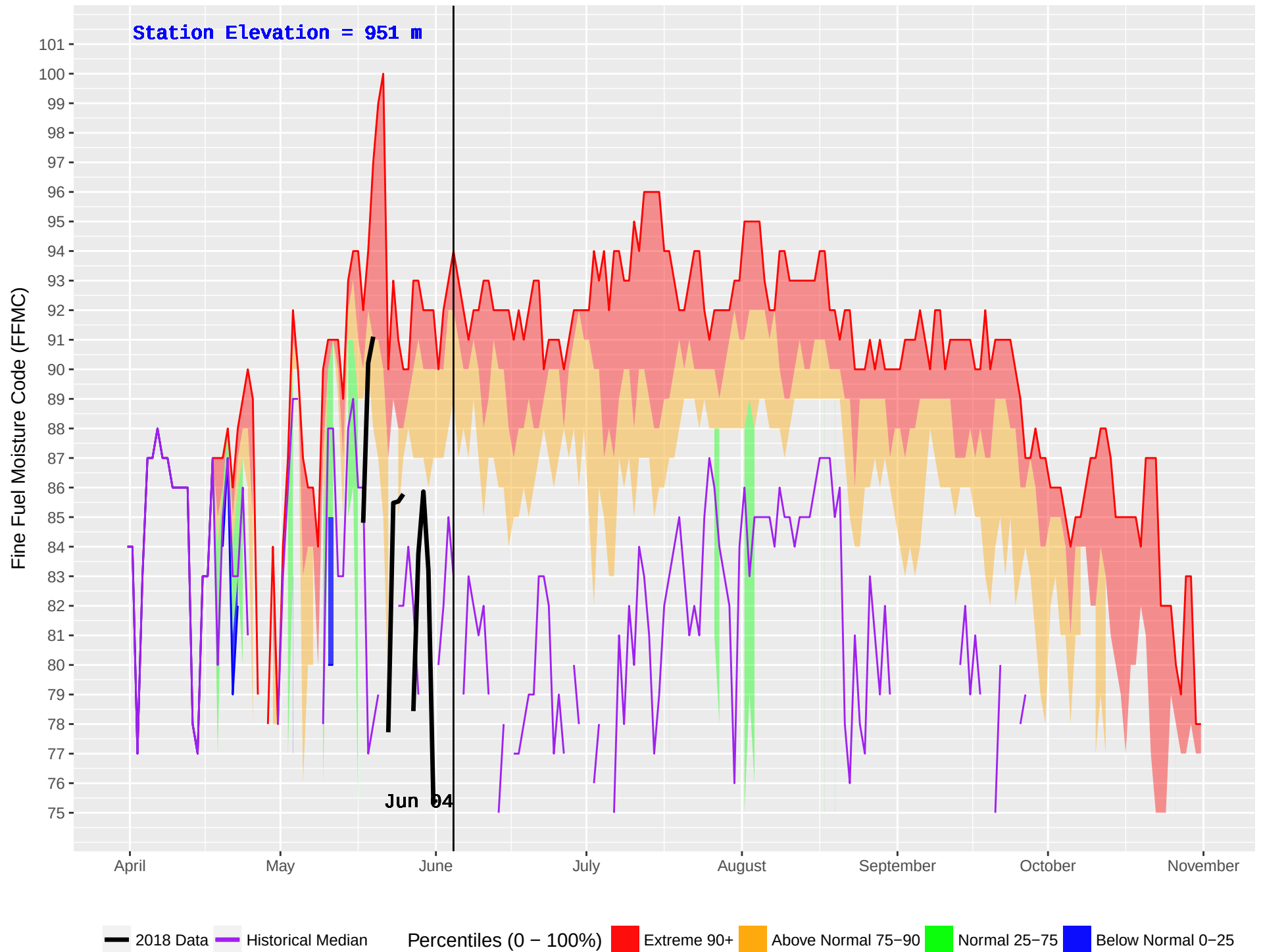
NORTH BABINE (173) : Historical (1986–2016) and Current (2018) Noon Fine Fuel Moisture Code (FFMC)
