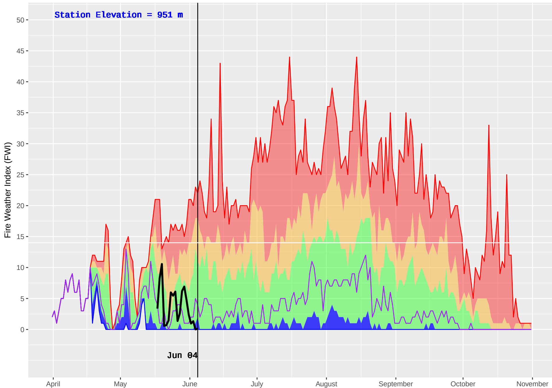
NORTH BABINE (173) : Historical (1986–2016) and Current (2018) Noon Fire Weather Index (FWI)
