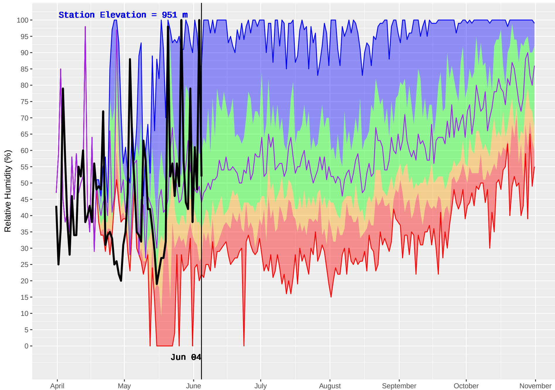
NORTH BABINE (173) : Historical (1986–2016) and Current (2018) Noon Relative Humidity
